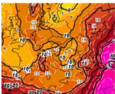
Fig. 16. The surface-level air isobaric temperature (°C) of 850 hPa on 11 July 2016 at Available Potential Energy (CAPE) on 11 July 2011, 12 UTC (Source: www.wetter3.de )
