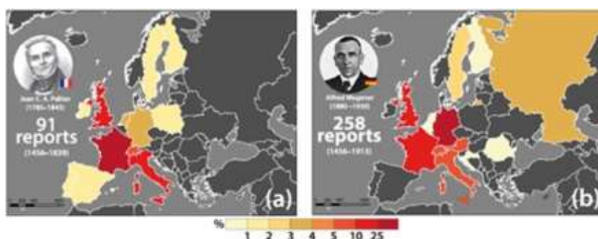
Fig.1. Spatial distribution of tornadoes reported over continental Europe between 1456 and 1839 (a) and between 1459 and 1913 (b) (Antonescu, 2016)
