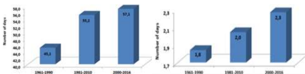
Fig. 8. Periodically number of days with shower days (left) and number of days with precipitation \geq 30 mm per day (right) overall Moldavian territory (1961 – 2016)
