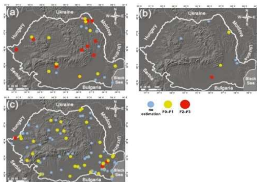
Fig. 6. Spatial distribution of tornadoes reported in Romania in different time periods(a) - historical tornadoes (33 reports between 1822 and 1944); (b) - tornado reports in the socialist period (seven reports between 1945 and 1989) and (c) – late tornado reports (89 reports between 1990 and 2013). In Romania, the tornadoes were classified according to their intensity on Fujita scale: weak tornado (F0 or F1 in yellow) and significant tornadoes (F2 and F3 in red).
