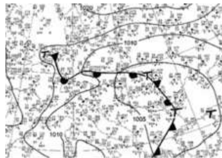
Fig. 15. Synoptic situation on 11 July 2014, 12 UTC at ground level
