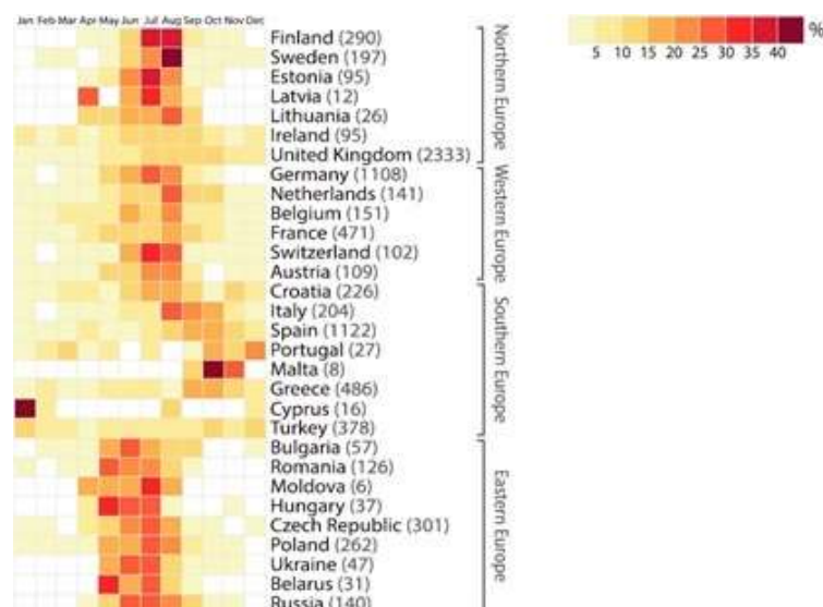
Fig. 3. Monthly distribution of tornadoes reported over continental Europe (Antonescu, B, 2016). Each cell represents the monthly percentage of the total number of tornadoes reported in each country (shown in brackets)
