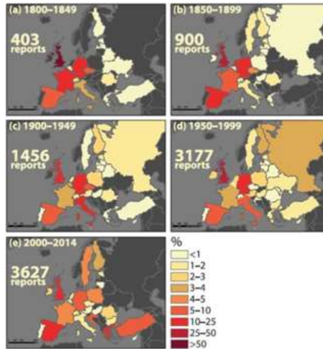
Fig.2. Spatial distribution of tornadoes reported over continental Europe in different time periods (Antonescu, 2016)
