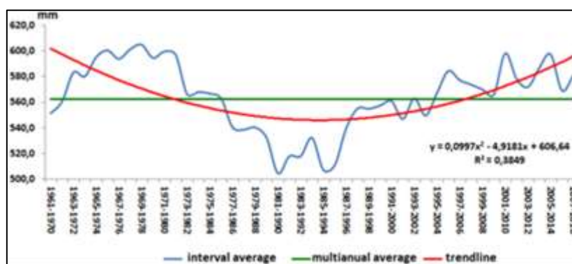
Fig. 7. The moving averages over a 10-year time series, shifted successively with one year of the annual average precipitation amounts overall Moldavian territory (1961 – 2016)
