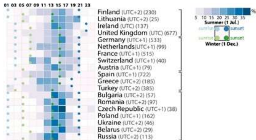
Fig. 4. Daily distribution of tornadoes reported over continental Europe (Antonescu, B, 2016). The local solar time for each country is shown in the first set of brackets. The total number of reports containing the time of occurrence is shown in the second set of brackets. Each cell represents the percentage of the total number of tornadoes reported in each country. The dots represent the sunrise and sunset in summer (blue) and winter (green)
