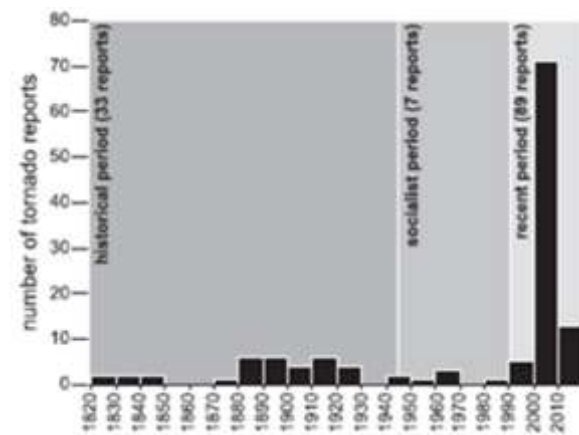
Fig. 5. Time distribution of tornadoes reported in Romania between 1822 - 2013 (first decade includes the years 1822 to 1829 and the last decade, the years 2010-2013)- Antonescu, 2015-
